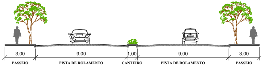
VIA ARTERIAL INTERNA = 25,00m
